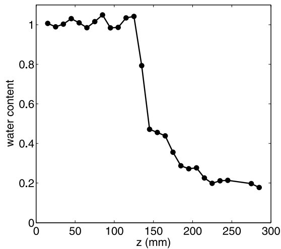
Figure 7. Water content versus height in the column after infiltrations (with colloids or without). Water is retained at the bottom of the column because of capillary forces, and the curve resembles the soil characteristic curve.
