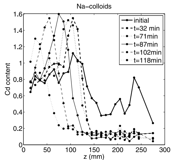
Figure 10. Na colloid content versus space and time for a slow flush with DI water. The colloid content forms a bank at the leading edge of the displacing water. This bank has colloid content over 60% higher than the initial infiltrating mixture.
