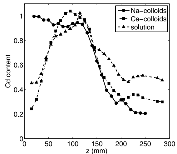
Figure 8. Cd content versus height during the initial infiltration for Cd attached to Na and Ca colloids and for Cd in solution. The Cd in solution is retained the most, while the Cd content for the Na colloids basically matches the water saturation (in other words, all the Na colloids are still in solution). The Cd content for the Ca colloids is basically between the two. Note that the drop-off in content near z = 0 for the Ca and Cd in solution is due to the Cd front being retarded with respect to the saturation front.
