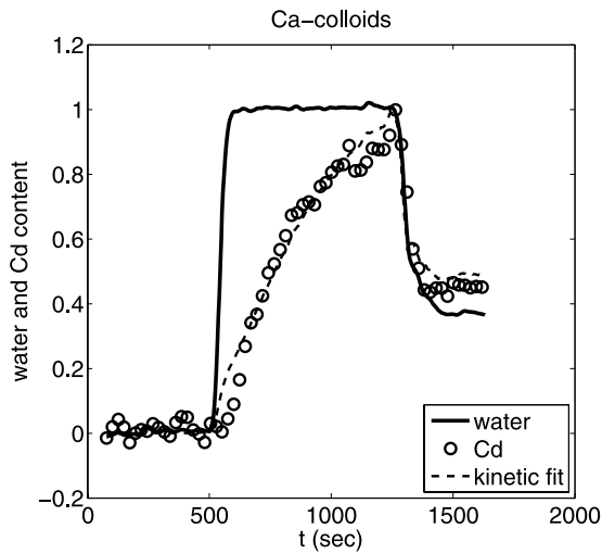
Figure 5a. Trace of normalized water and Cd content versus time where the Cd is attached to the Ca colloids. The infiltrating flux was 0.26 cm/min, and the observation was made 60 mm below the sand pack surface. The water content shows similar behavior to the infiltration using the Na colloids, but the Cd content (attached to the Ca colloids) shows a delayed response with respect to the water.
