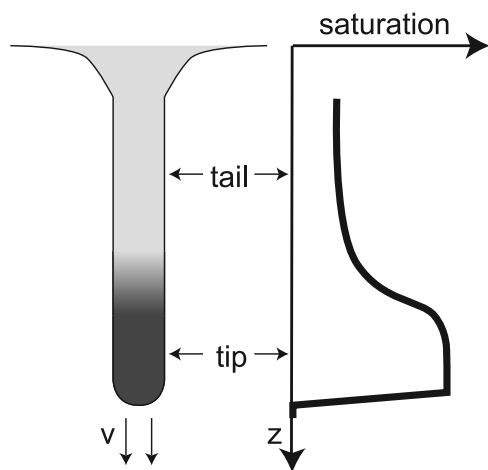
Figure 1. Cartoon of a preferential flow path and the associated saturation within the flow path. Preferential flow creates a unique saturation profile with saturated conditions at the tip and unsaturated conditions in the tail. Colloid retention may be affected by the fast moving water/air interfaces.
