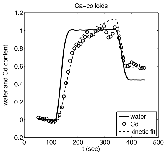
Figure 5b. Trace of normalized water and Cd content versus time where the Cd is attached to Ca colloids. At a higher flux of 1.28 cm/min the behavior is very similar to that seen at the lower flux (Figure 5a).
