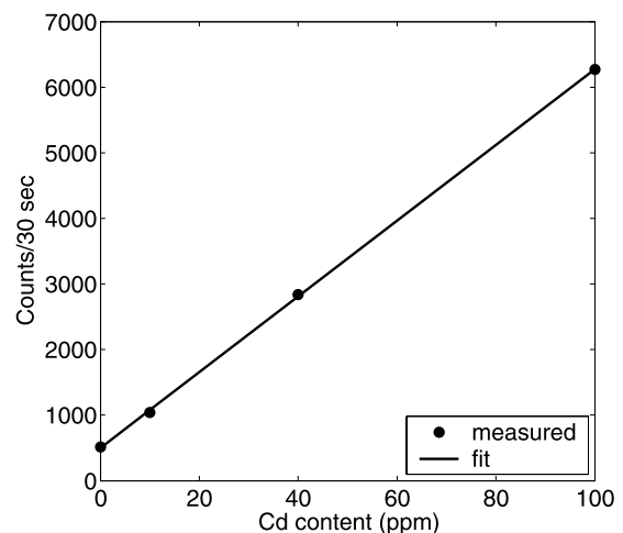
Figure 3. Calibration curve for the Na colloids with Cd attached. The Cd content can be determined to an accuracy of 2 mg/L for a 10 s counting time.
