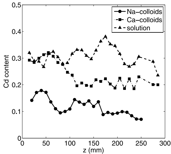
Figure 9. Cd content versus height after two flushes of two pore volumes of DI water for Cd attached to Na and Ca colloids and for Cd in solution. Again the Cd content observed is greatest for the Cd in solution and least for the Cd attached to the Na colloids. After the two flushes, the retention of the colloids is relatively constant versus height, with no significant difference between the saturated zone ( z < 150 mm) and the unsaturated zone ( z > 150 mm).
