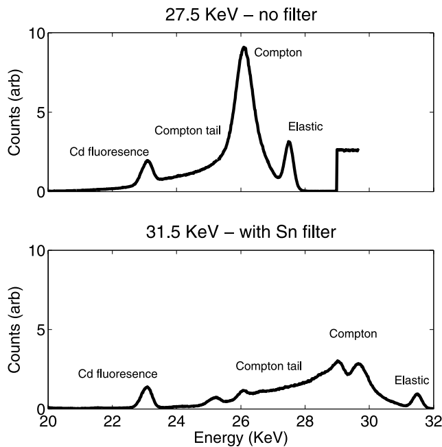
Figure 2. X-ray spectrum measured with the Si detector with a sample of 100mg/L Cd in the sample position. The top spectrum is the spectrum obtained with incident X rays of sufficient energy to elicit fluorescence of the Cd, but it has much Compton scattering in the Cd fluorescence window. The bottom spectrum is the one used during the experiment with a higher-energy incident X ray and a Sn filter with much lower background counts.
