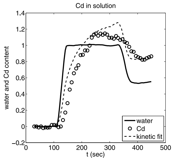
Figure 6b. Trace of normalized water and Cd content versus time where the Cd is in solution for a higher flux of 1.28 cm/min. The behavior is very similar to that seen at the lower flux (Figure 6a).
