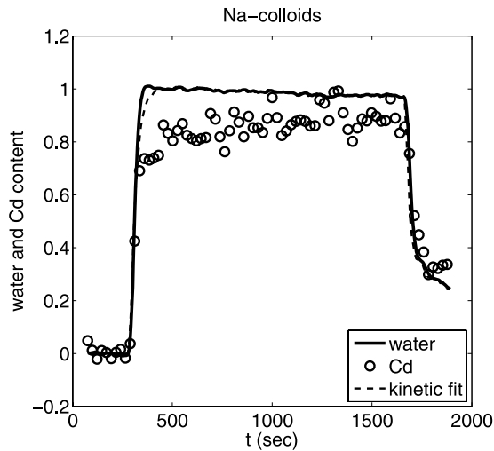
Figure 4a. Trace of normalized water and Cd content versus time where the Cd is attached to the Na colloids. The infiltrating flux was 0.26 cm/min, and the observation was made 60 mm below the sand pack surface. The Cd content follows the water content at all times showing that there is no appreciable retention of the Na colloids.
