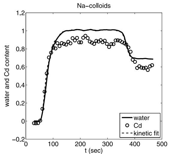
Figure 4b. Trace of normalized water and Cd content versus time where the Cd is attached to Na colloids. At a higher flux of 1.28 cm/min, the behavior is very similar to that seen at the lower flux (Figure 4a).
