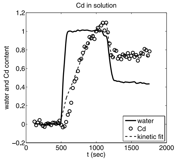
Figure 6a. Trace of normalized water and Cd content versus time where the Cd is in solution. The infiltrating flux was 0.26 cm/min, and the observation was made 60 mm below the sand pack surface. Again the water content behavior is similar to the other infiltrations. For the Cd in solution a delayed response with respect to the water is observed, similar to that seen for the Cd attached to the Ca colloids.
